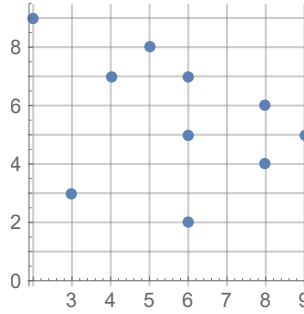
Slika 9.6: Skup \mathcal{A} = \{(2,9), (3,3), (4,7), (5,8), (6,2), (6,5), (6,7), (8,4), (8,6), (9,5)\}
